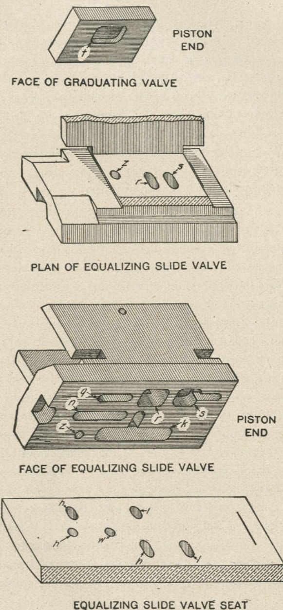
FIG. 362. Views of the Equalizing Valve, Graduating Valve and Equalizing Valve Seat.
