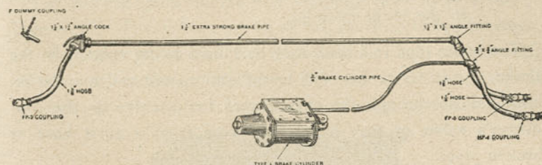
FIG. 356. Piping Diagram of Tender Brake Equipment.
