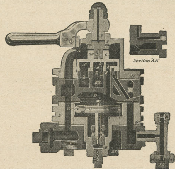
FIG. 365. Section of H-6 Automatic Brake Valve.
