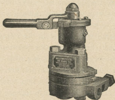
FIG. 367. S-6 Independent Brake Valve.
