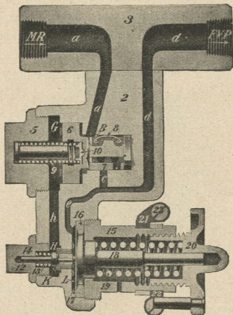
FIG. 371. Diagram of B-6 Feed Valve, Closed.
