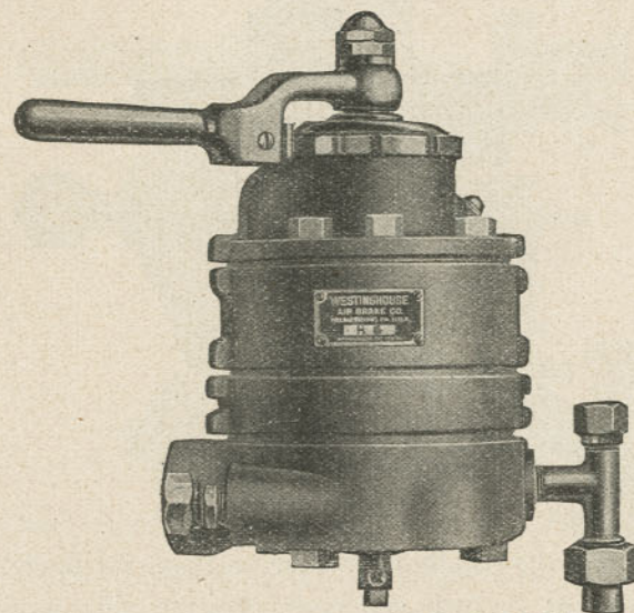
FIG. 363. H-6 Automatic Brake Valve.
