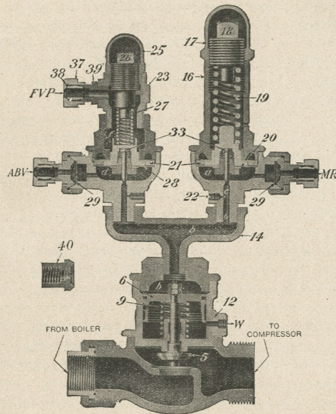
FIG. 374. Type SF Compressor Governor.
