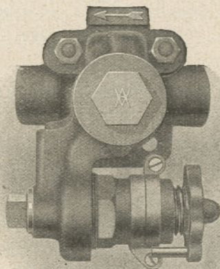
FIG. 370. B-6 Feed Valve and Bracket, Complete.
