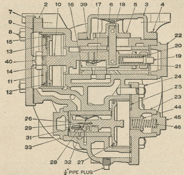
FIG. 359. Sectional View of No. 6 Distributing Valve.
