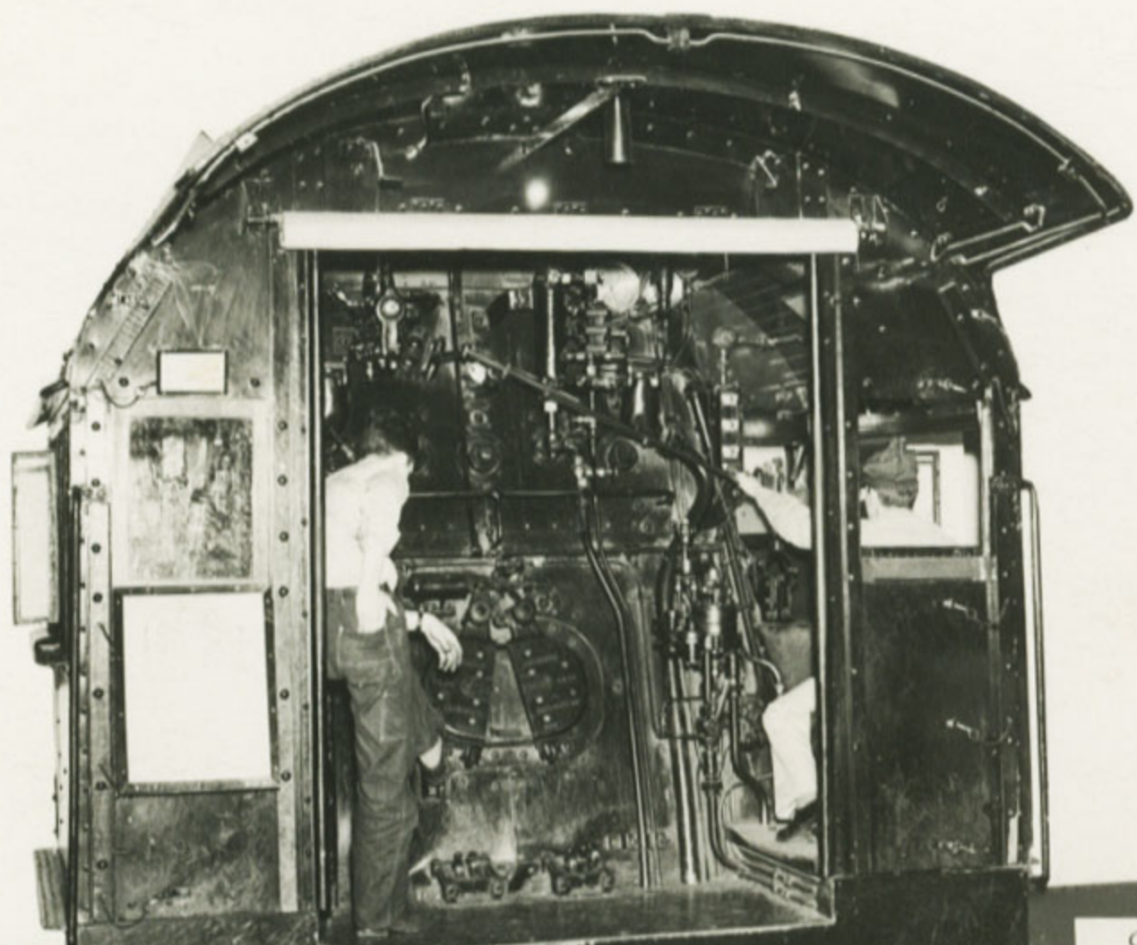
LOCOMOTIVE CAB
