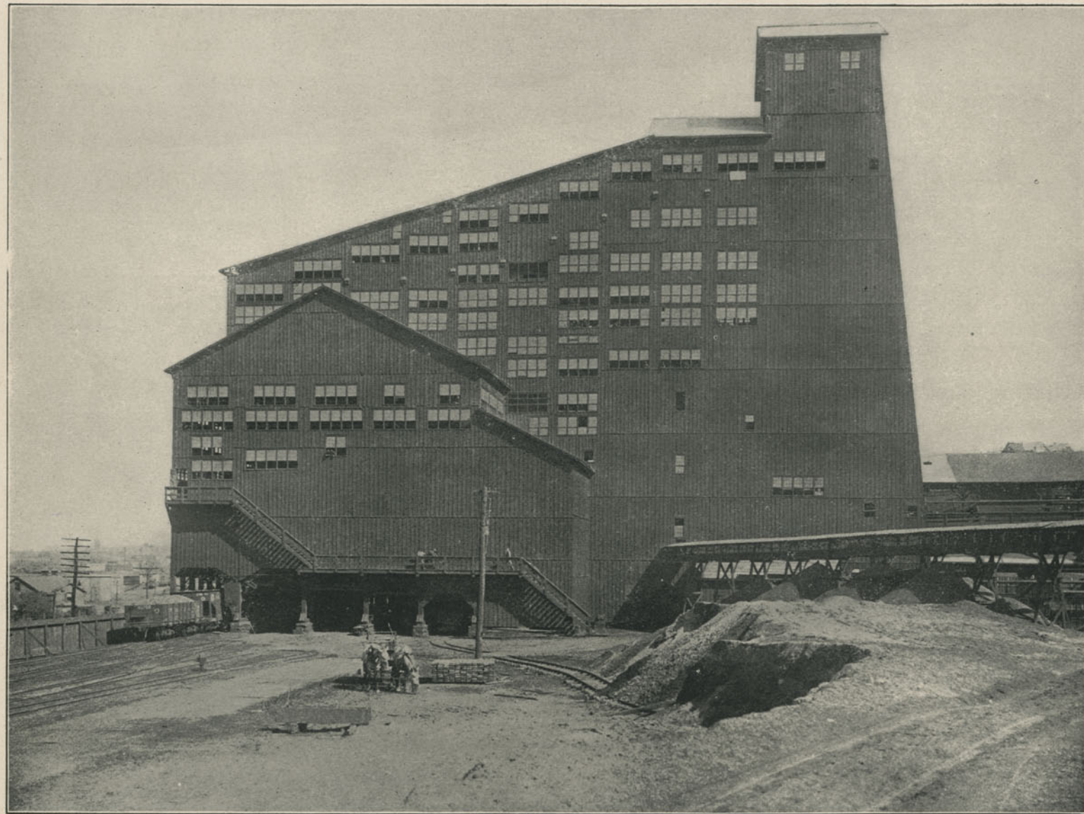
COAL BREAKER
