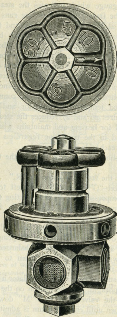
FIG. 26. IMPROVED TEMPERATURE REGULATOR.
