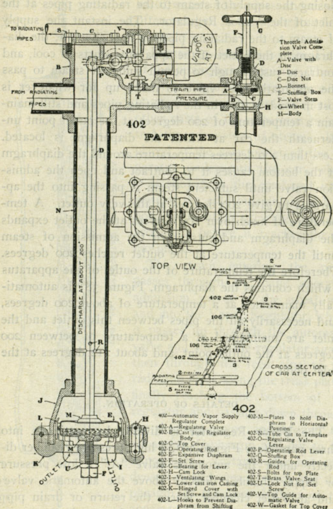
FIG. 39. DETAILS OF VAPOR REGULATOR.
