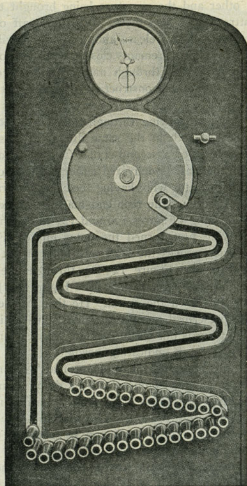
FIG. 127. ABSOLUTE STAFF INSTRUMENT.
