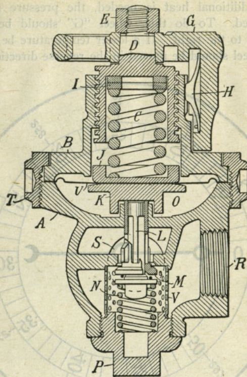
FIG. 27. SECTIONAL VIEW IMPROVED TEMPERATURE REGULATOR.
