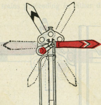
FIG. 104. A THREE-POSITION SIGNAL. "STOP"-HORIZONTAL; "CAUTION"-UP; "PROCEED"-DOWN.
