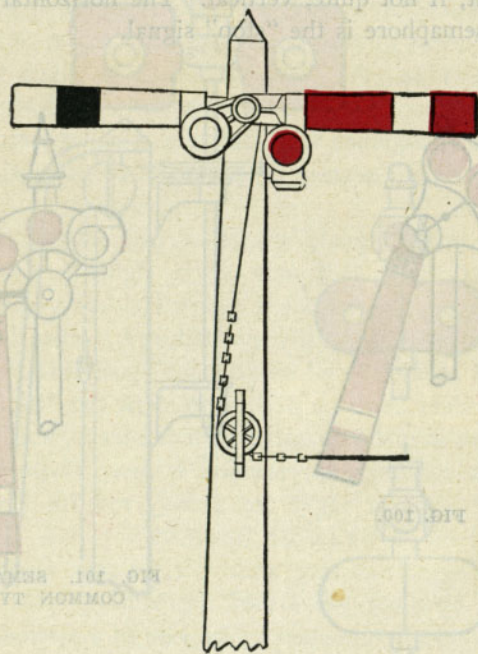
FIG. 102. A TWO-POSITION TRAIN-ORDER SIGNAL.
