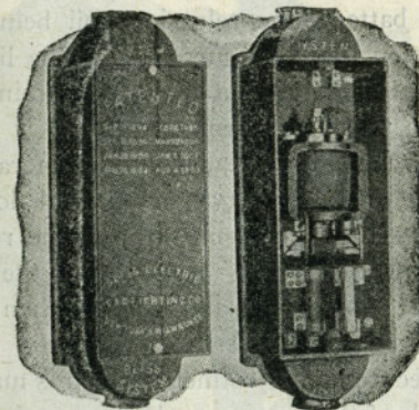
FIG. 94. GENERATOR SWITCH IN SINGLE SECTION IRON BOX.
