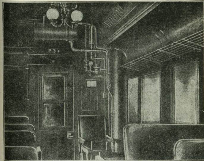
FIG. 59. INTERIOR OF COACH, WITH GAS GENERATOR INSTALLED.
