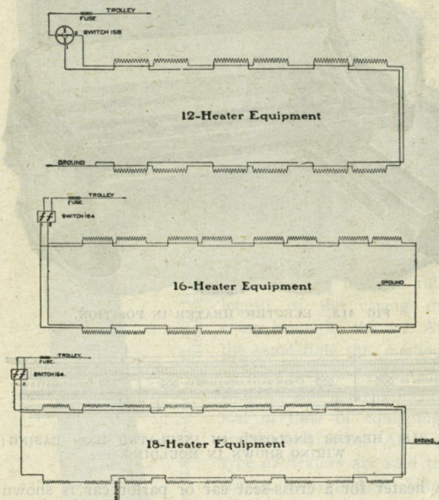
FIG. 42. DIAGRAMS OF WIRING ELECTRIC HEATING SYSTEM.
