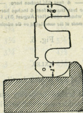
Method of Gauging Worn Flanges. See Rule 10.
