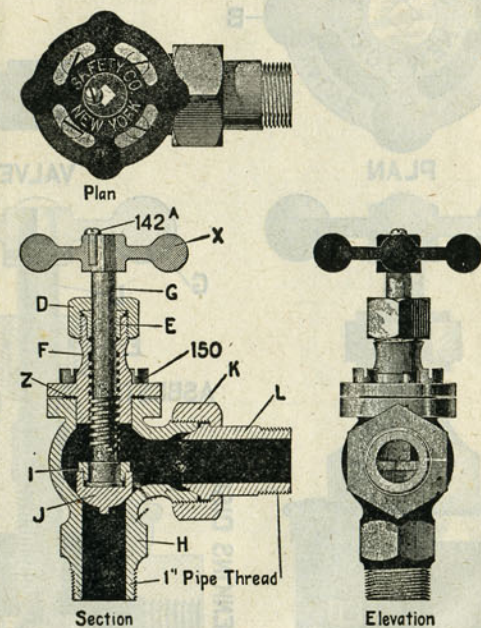
FIG. 15. ANGLE VALVE. (Used on Locomotive.)
