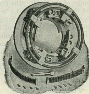
FIG. 86. AUTOMATIC BRUSH MECHANISM AND FLEXIBLE CABLES.
