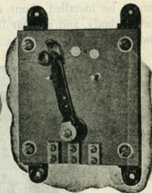
FIG. 97. EMERGENCY EXCITER SWITCH.
