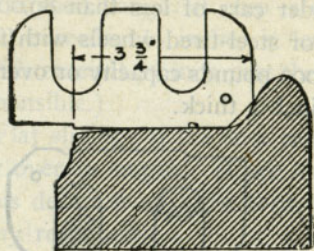
Method of Gauging Chipped Rings. See Rules 15 and 20.
