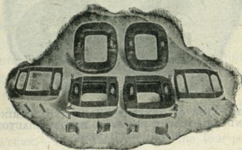
FIG. 81. GENERATOR FIELD COILS AND RETAINERS.
