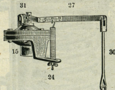
FIG. 5. AUTOMATIC REGULATOR AND PRESSURE INDICATOR.
