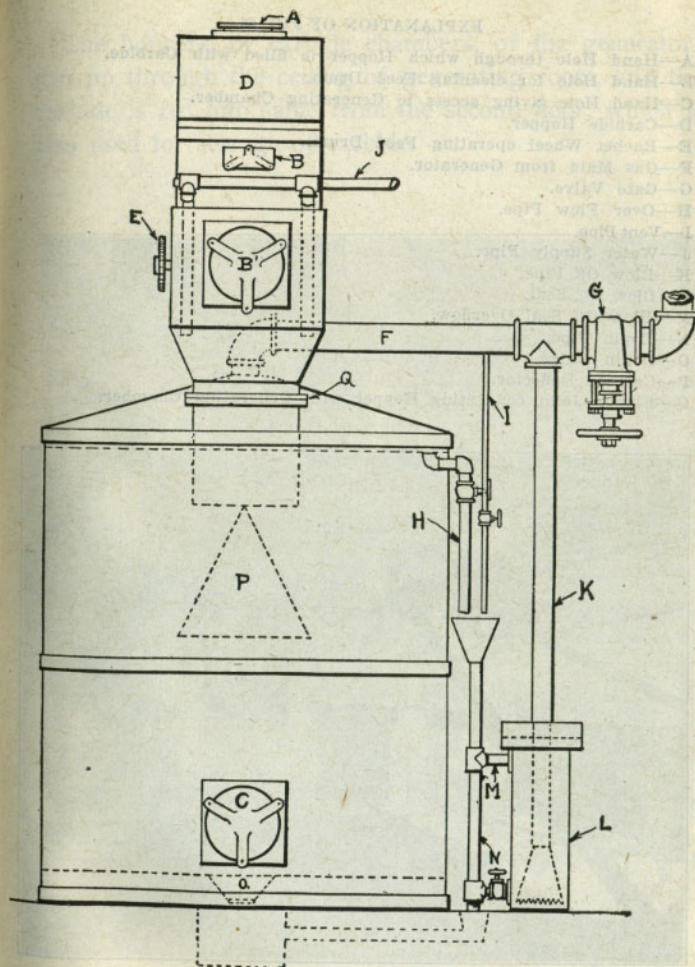
FIG. 66. GENERAL ACETYLENE GENERATOR.
