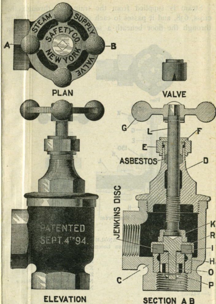
FIG 14. STEAM INLET VALVE.
