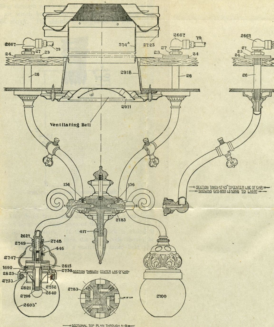
FIG. 55. SECTIONAL VIEW OF LAMP—DETAILS AND PARTS SHOWN.
