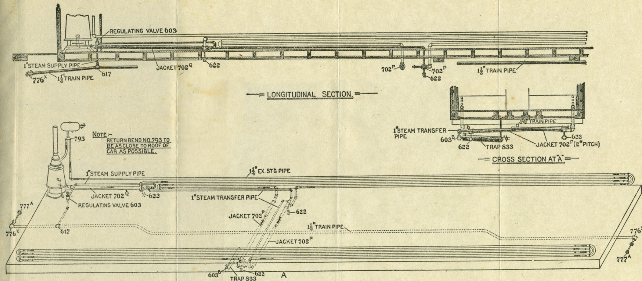
PLATE 1. Design showing Standard Heating System as used with Single Circulation Baker Heaters.
