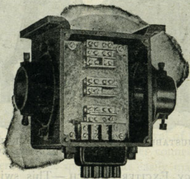
FIG. 98. FRONT VIEW JUNCTION BOX, WITH COVER REMOVED.
