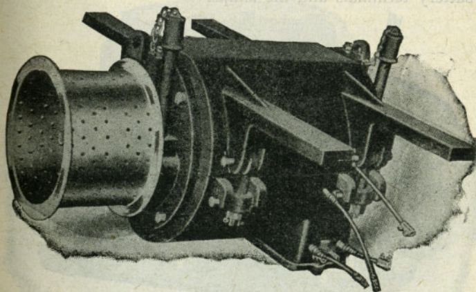
FIG. 73. GENERATOR SHOWING PERFORATED PULLEY AND SUPPORTING ARMS.
