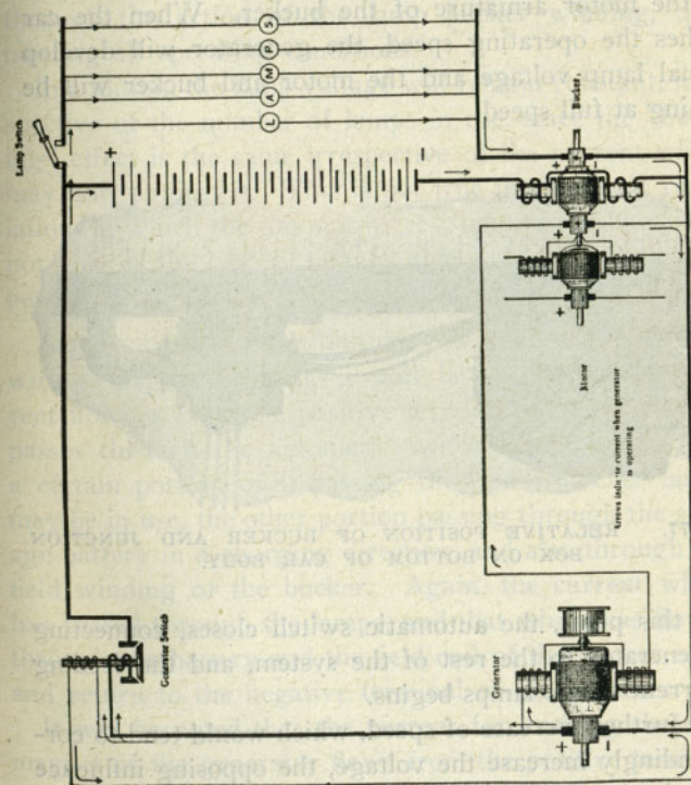
FIG. 76. PARTIAL THEORETICAL WIRING DIAGRAM.
