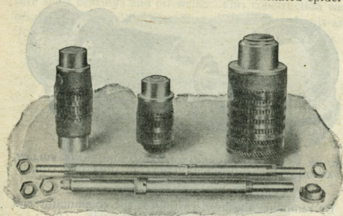
FIG. 84. ARMATURE SHAFTS AND NUTS OF GENERATOR AND BUCKER, SHOWING SPIDER AND REMOVABLE SHAFT CONSTRUCTION.
