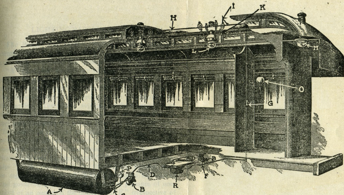
GENERAL ARRANGEMENT OF APPARATUS ON A CAR
