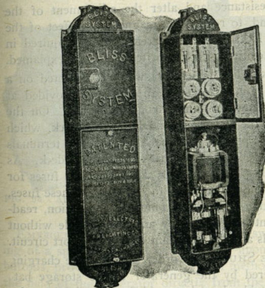
FIG. 95. GENERATOR SWITCH WITH FOUR-CIRCUIT PANEL BOARD IN DOUBLE SECTION IRON BOX.
