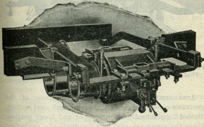
FIG. 78. CAR GENERATOR SHOWING OUTSIDE SUSPENSION, PULLEY END.
