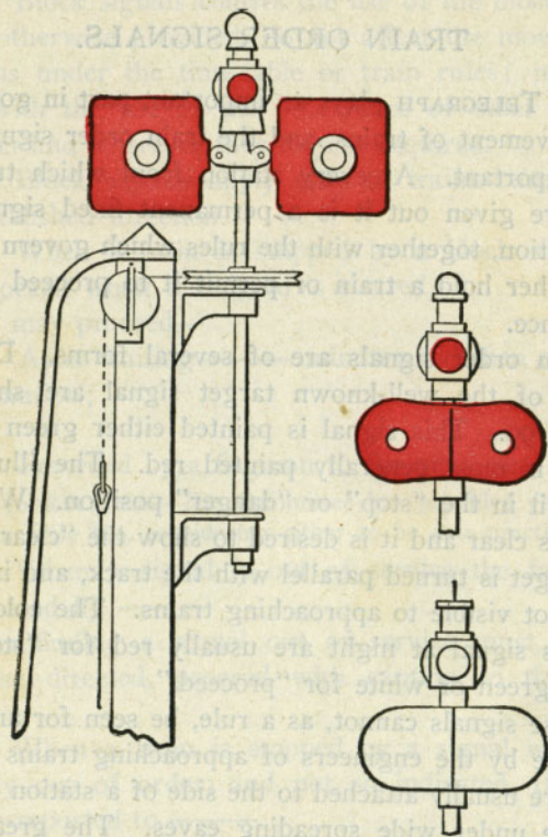
FIG. 99. TARGET SIGNALS.
