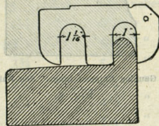
Method of Gauging Worn Flanges. See Rule 10.
