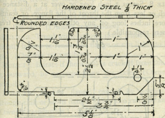
Worn Coupler Limit and Wheel Defect Gauge.
