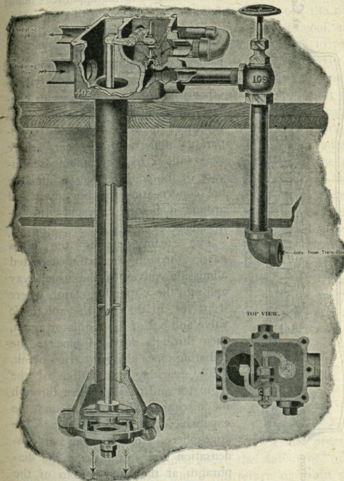
FIG. 37. VAPOR HEATING—SECTIONAL VIEW.
