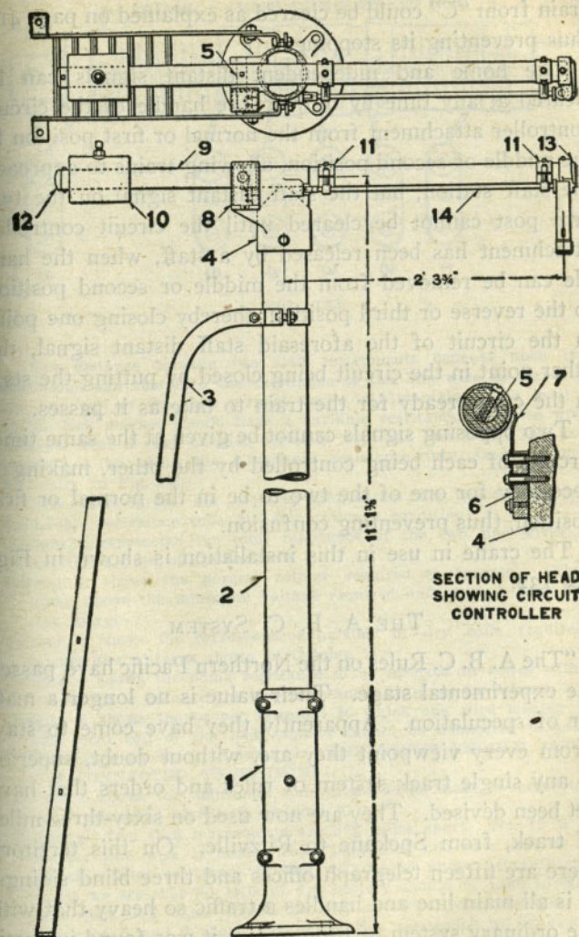
FIG. 132. CRANE STAFF DELIVERER.
