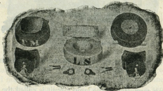
FIG. 89. BUCKER FIELD COILS AND POLE PIECES.
