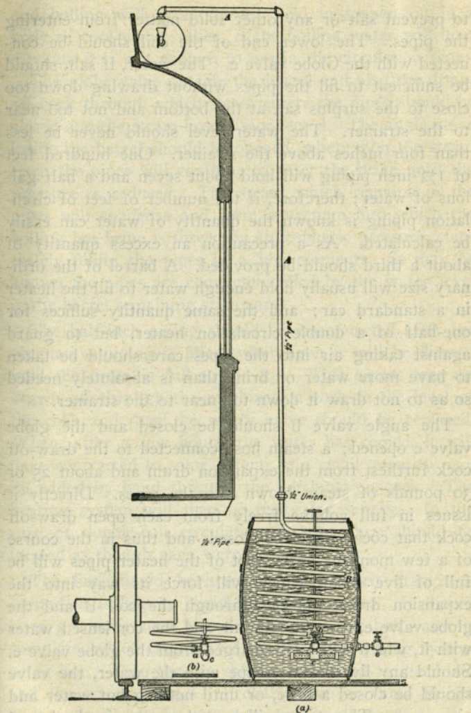
FIG. 7. ARRANGEMENT ILLUSTRATING METHOD OF FILLING THE HEATER CIRCULATION SYSTEM.
