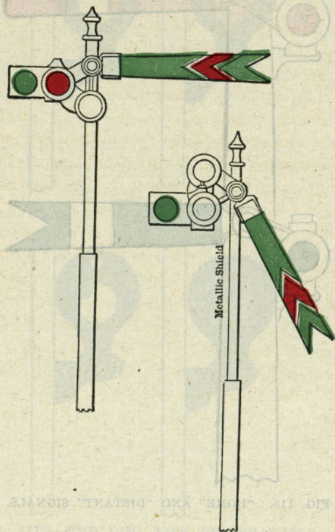
FIG. 119. "CLEAR" INDICATED BY GREEN LIGHT.
