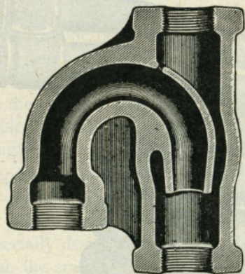
FIG. 32B. SECTIONAL VIEW DUPLEX COILS.
