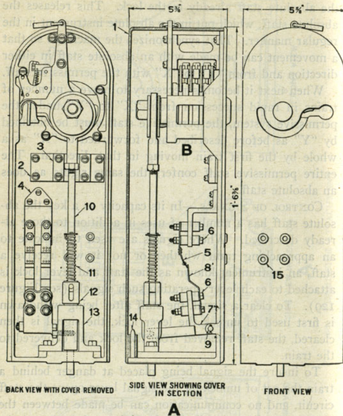
FIG. 129. STAFF LEVER LOCK.
