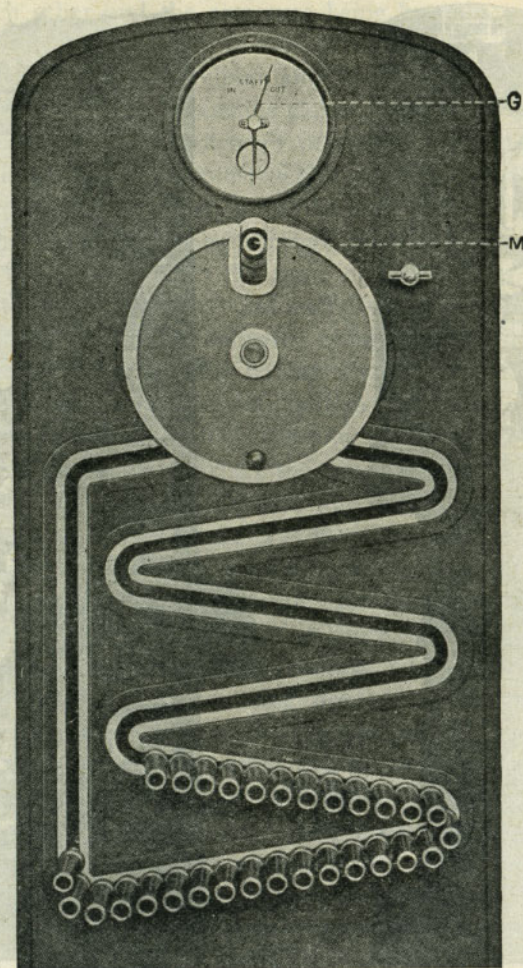
FIG. 124. ABSOLUTE STAFF INSTRUMENT.
