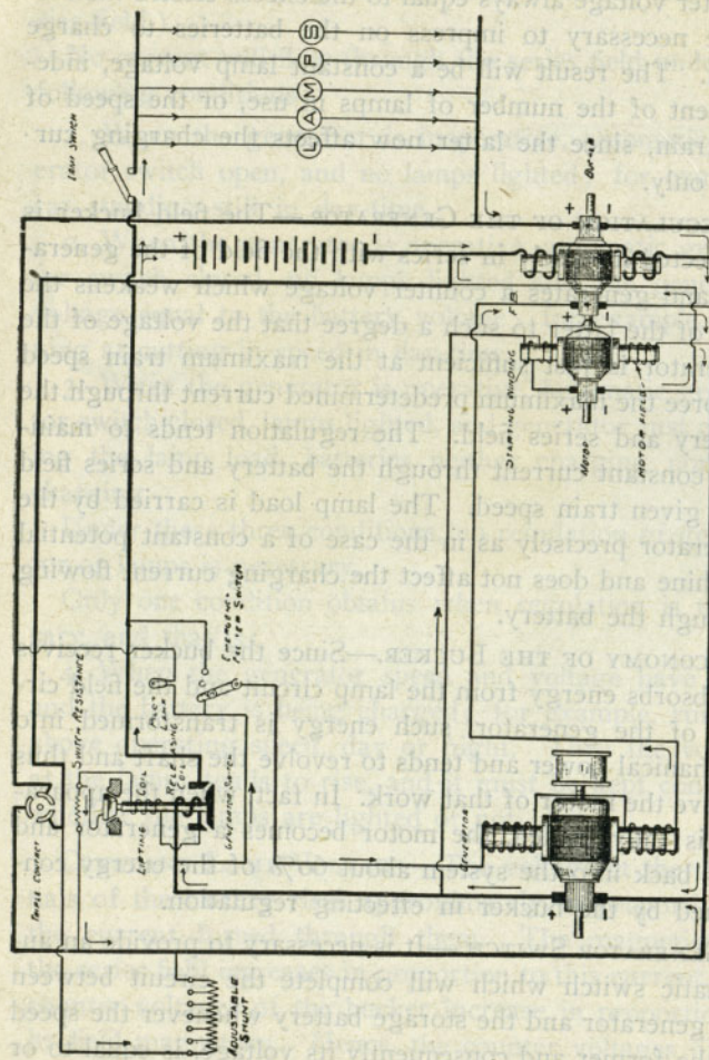
FIG. 93. COMPLETE THEORETICAL WIRING DIAGRAM.
