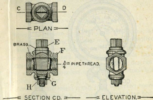
FIG. 16. REDUCING VALVE. (Used on Locomotive.)
