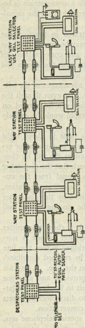
Diagram Indicating Method of Cutting Stations into Telephone Circuit for Dispatcher's Use.
