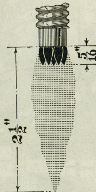
FIG. 56. SHOWING PROPER FLAME.
