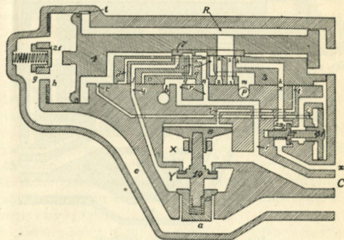
FIG. 355. GRADUATED-RELEASE-LAP POSITION
