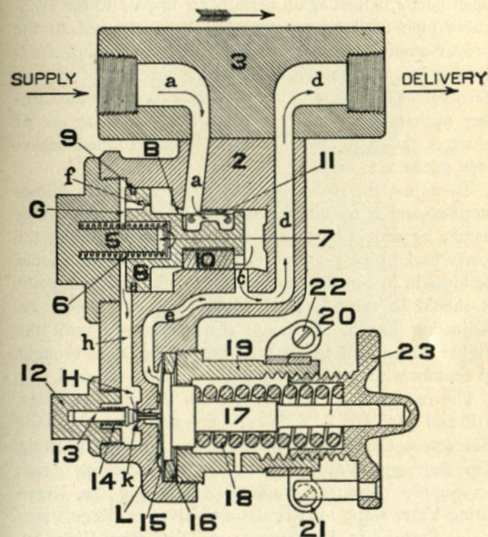
FIG. 319. DIAGRAM OF FEED VALVE, OPEN
