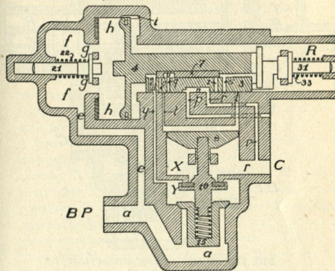
FIG. 326. FULL-RELEASE AND CHARGING POSITION
