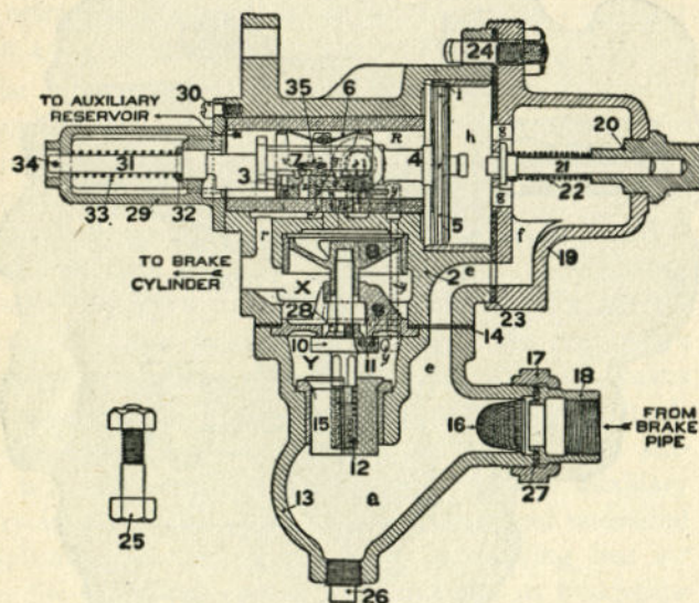
FIG. 324. THE K-2 TRIPLE VALVE
