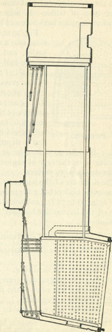
FIGURE 29. SECTION OF MODERN BOILER
