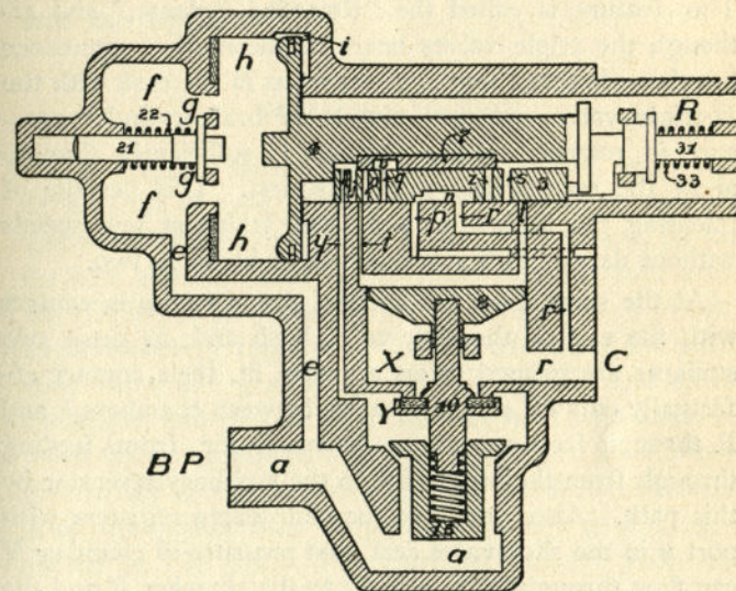
FIG. 330. RETARDED-RELEASE POSITION
