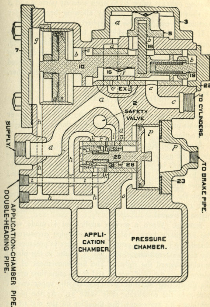
FIG. 301. INDEPENDENT LAP
