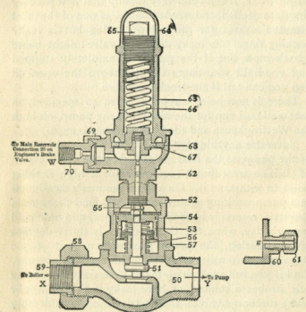
FIGURE 226 PUMP GOVERNOR
