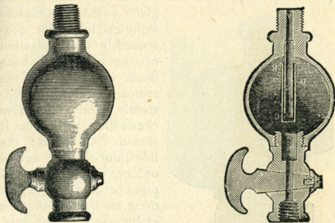
FIGURE 193 PRINDLE'S PATENT SYPHON COCKS
