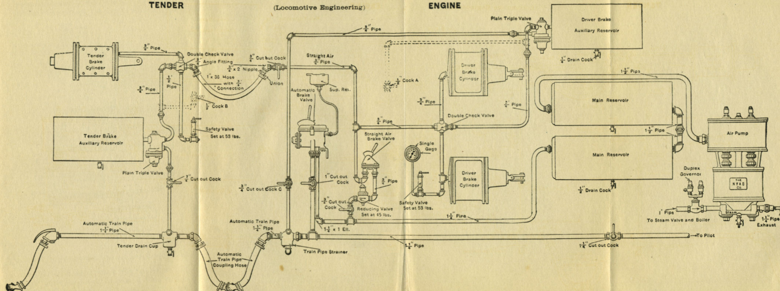
GENERAL ARRANGEMENT AND METHOD OF PIPING THE NEW YORK COMBINED AUTOMATIC AND STRAIGHT AIR BRAKE.
