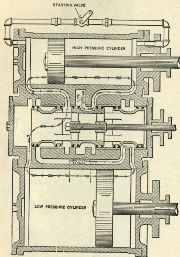
STEAM DISTRIBUTION IN BALANCED COMPOUND CYLINDERS.
