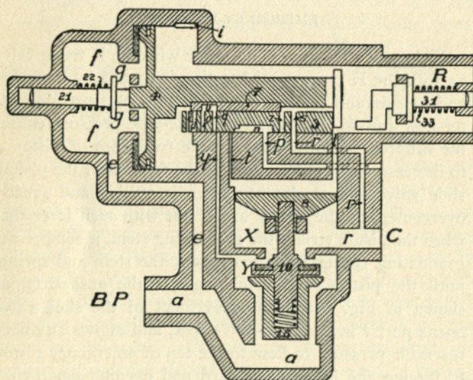
FIG. 331. EMERGENCY POSITION
