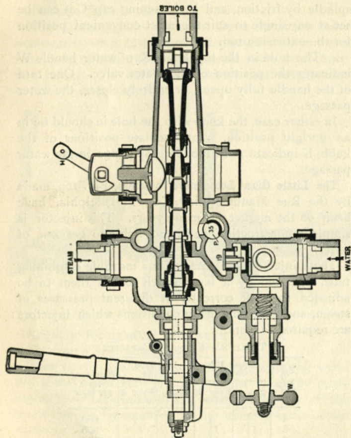
FIGURE 170 THE SIMPLEX INJECTOR
