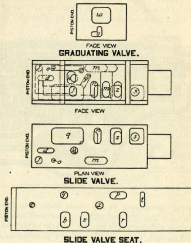
FIG. 350. GRADUATING VALVE, SLIDE VALVE, AND SLIDE-VALVE SEAT. TYPE L TRIPLE VALVE
