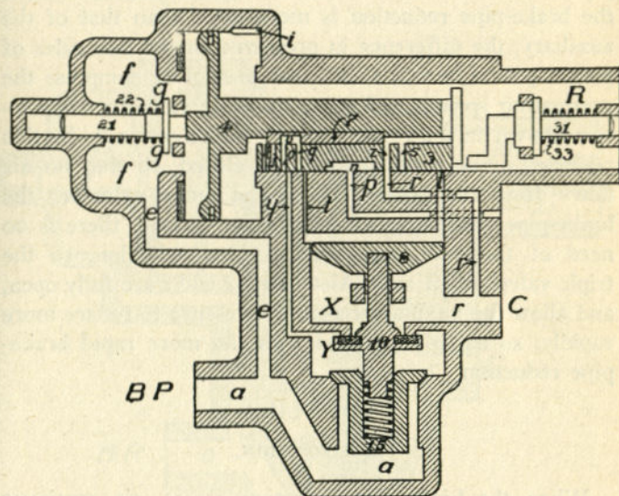
FIG. 328. FULL SERVICE POSITION
