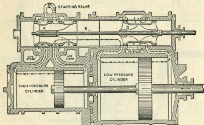
STEAM DISTRIBUTION IN TANDEM COMPOUND CYLINDERS
