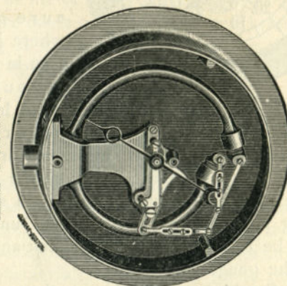
FIGURE 178 CROSBY LOCOMOTIVE PRESSURE GAUGE SECTIONAL VIEW
