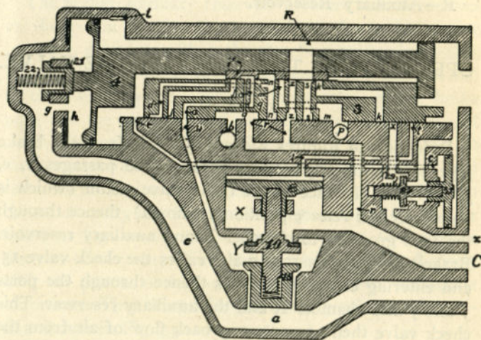
FIG. 352. QUICK-SERVICE POSITION
