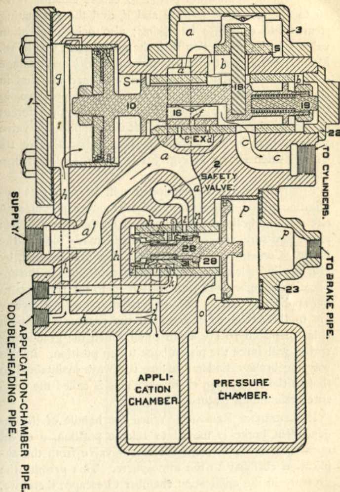
FIG. 300. INDEPENDENT APPLICATION
