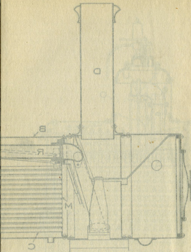
Fig. 6. Vertical Longitudinal Section of a Locomotive Boiler
