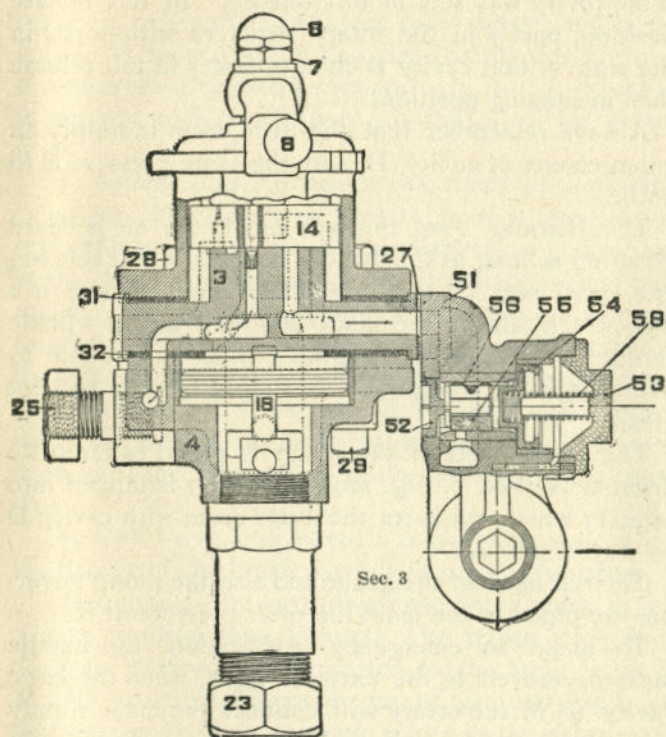
FIGURE 231 G-6 BRAKE VALVE
