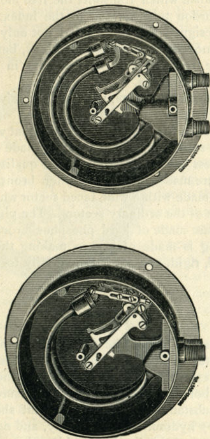
FIGURE 180 CROSBY DUPLEX GAUGE, SECTIONAL VIEW
