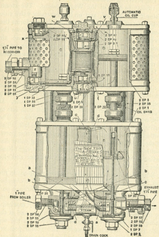
FIGURE 240 NEW YORK DUPLEX AIR PUMP, UPSTROKE, LOW-PRESSURE PISTON
