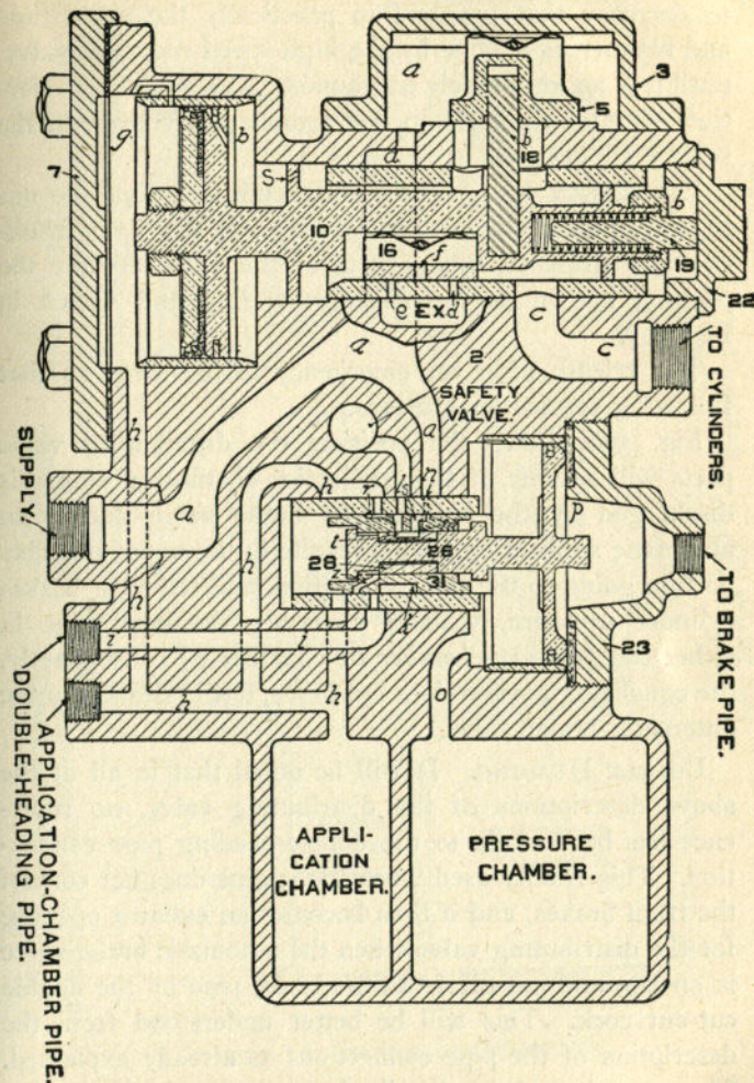
FIG. 305. EMERGENCY LAP
