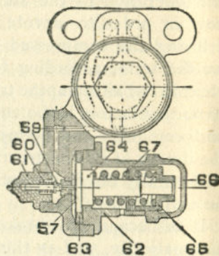
FIGURE 232 SLIDE VALVE FEED VALVE
