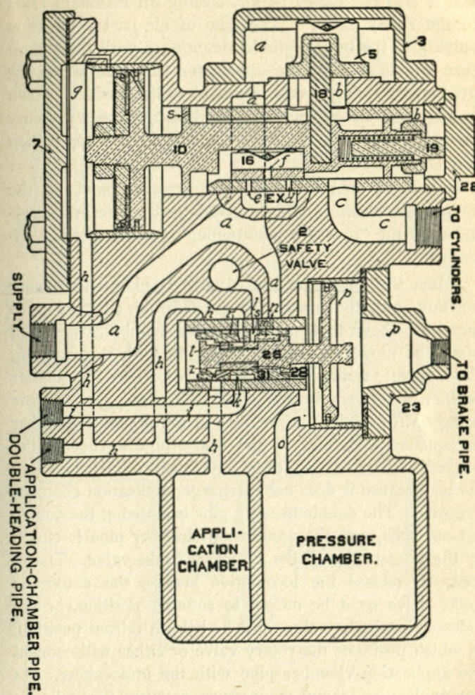
FIG. 303. SERVICE LAP
