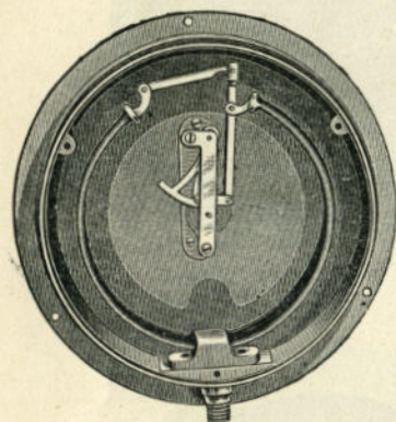
FIGURE 182 SECTIONAL VIEW AMERICAN PRESSURE GAUGE
