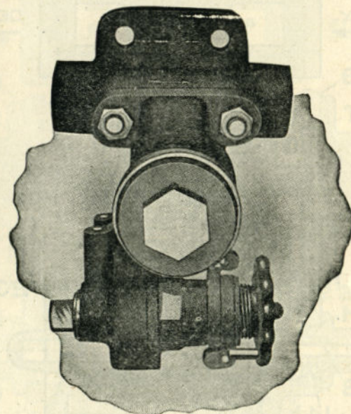
FIG. 317. FEED VALVE
