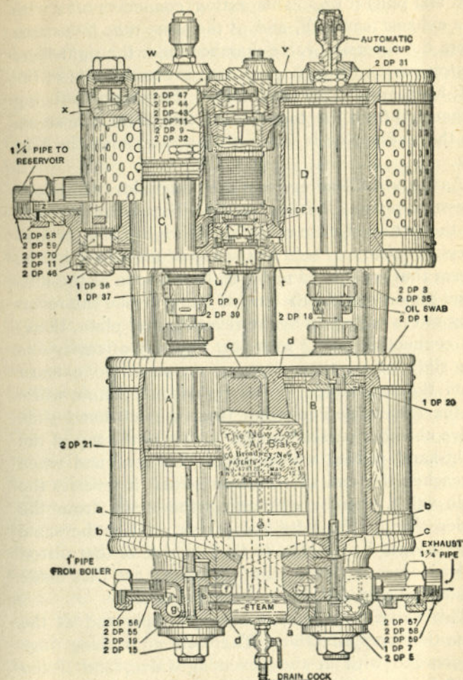
FIGURE 241 NEW YORK DUPLEX AIR PUMP UP STROKE, HIGH-PRESSURE PISTON
