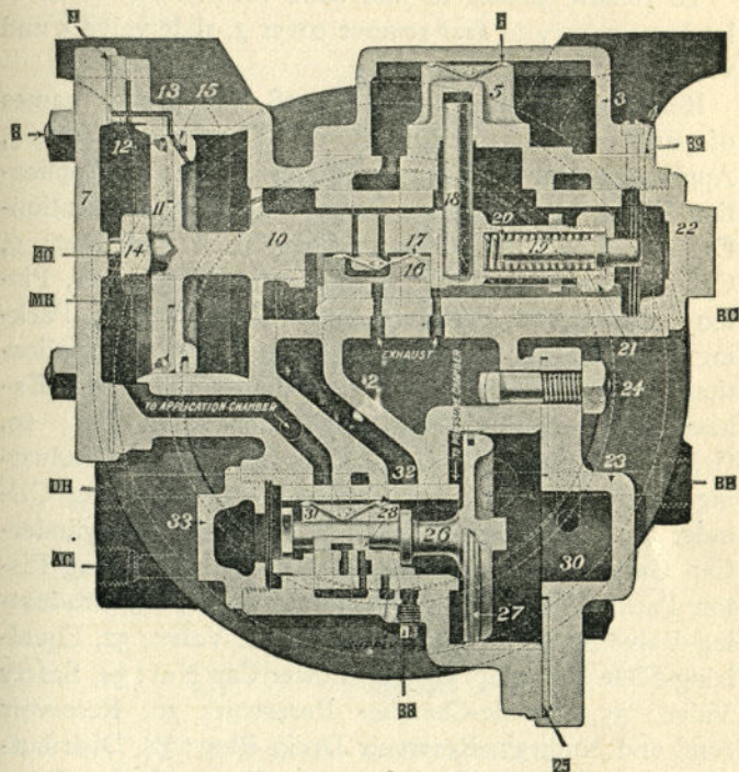
FIG. 308. DISTRIBUTING VALVE
