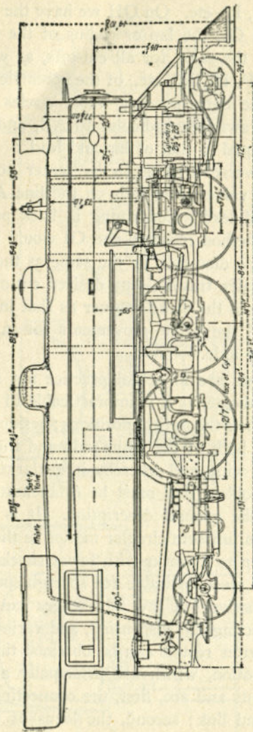
FIG. 341. WALSCHAERT VALVE GEAR—PRAIRIE TYPE PASSENGER LOCOMOTIVE—PENNSYLVANIA RAILROAD
