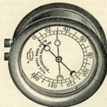
AMERICAN DUPLEX AIR-BRAKE GAUGE, WESTINGHOUSE STYLE
