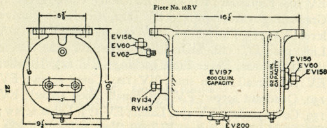
Fig. 279. Divided Reservoir.
