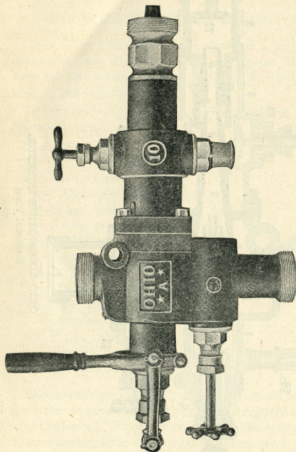
OHIO LOCOMOTIVE INJECTOR Lever Movement
