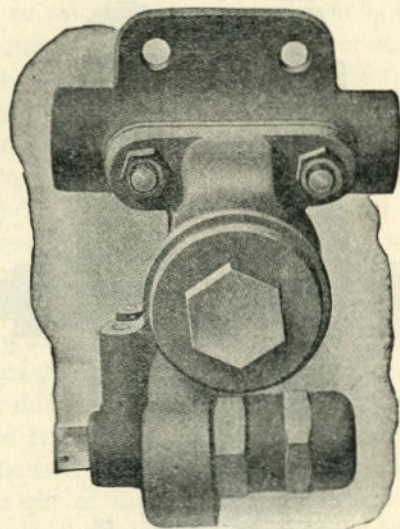
FIG. 320. REDUCING VALVE
