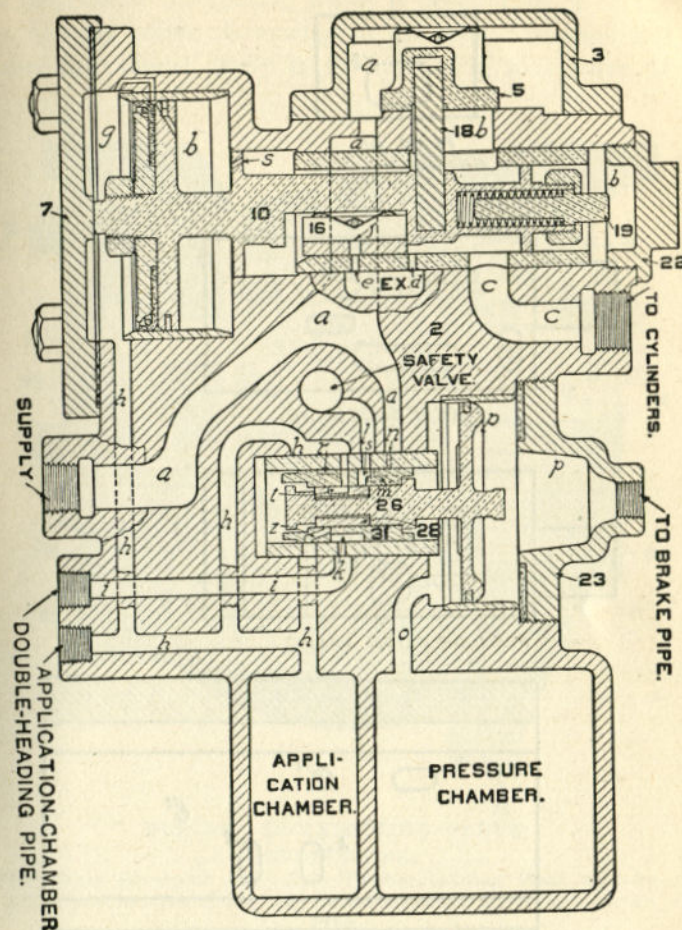
FIG. 306. RELEASE POSITION
