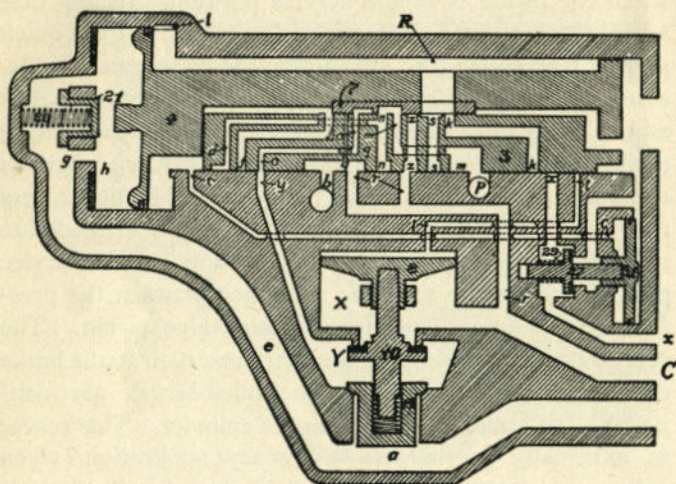
FIG. 354. SERVICE-LAP POSITION
