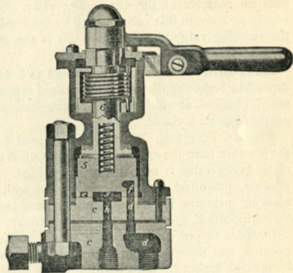
FIG. 315. INTERIOR VIEW OF THE INDEPENDENT BRAKE VALVE
