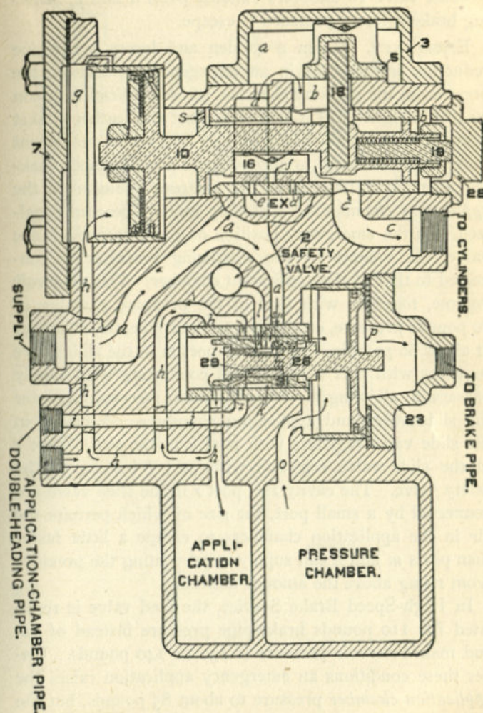
FIG. 304. EMERGENCY
