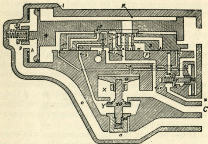
FIG. 353. FULL-SERVICE POSITION
