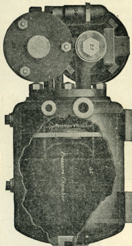
FIG. 297. DISTRIBUTING VALVE AND DOUBLE-CHAMBER RESERVOIR
