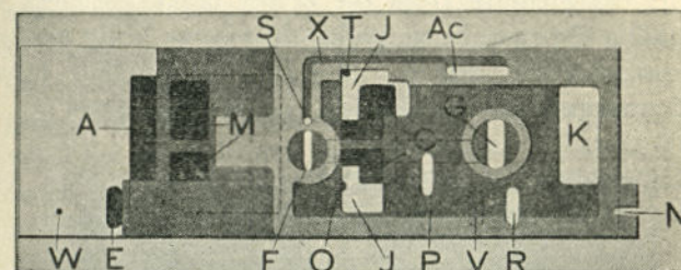
Fig. 272. Release Position.
