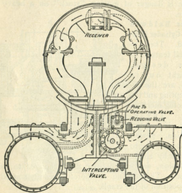
TWO-CYLINDER COMPOUND. CROSS-SECTION FIGURE 150
