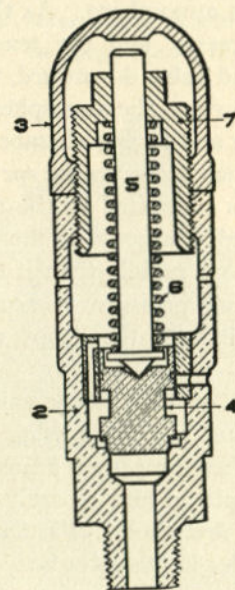
FIG. 309. SAFETY VALVE
