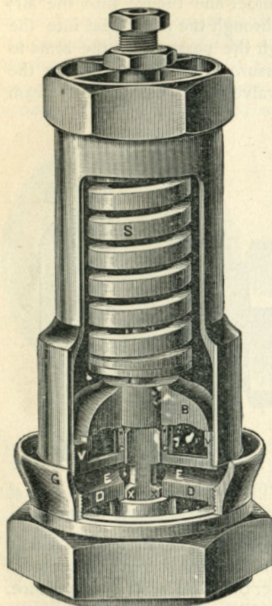
FIGURE 186 CROSBY LOCOMOTIVE POP SAFETY VALVE
