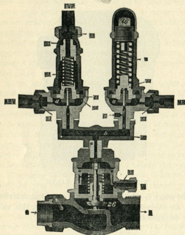
FIG. 321. PUMP GOVERNOR
