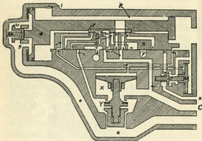
FIG. 356. EMERGENCY POSITION
